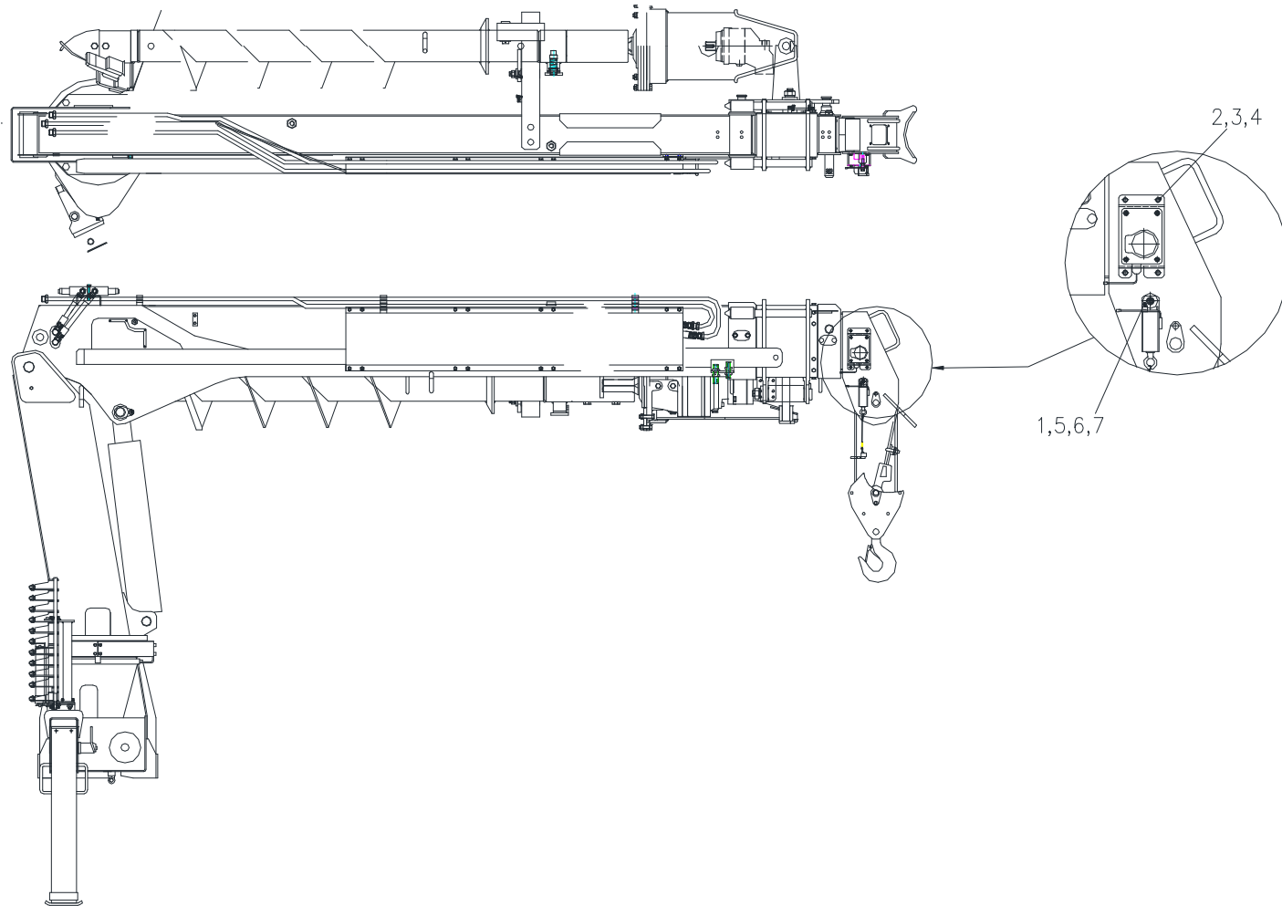
Fig. 11-1 SAC-2501R OVERWINDING ALARM SYSTEM
