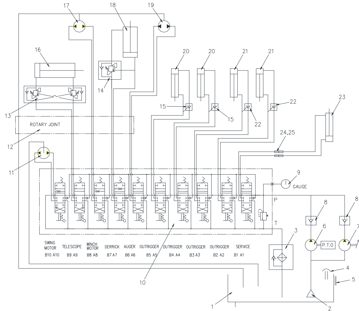
Fig. 10 SAC-2501R HYDRAULIC DIAGRAM
