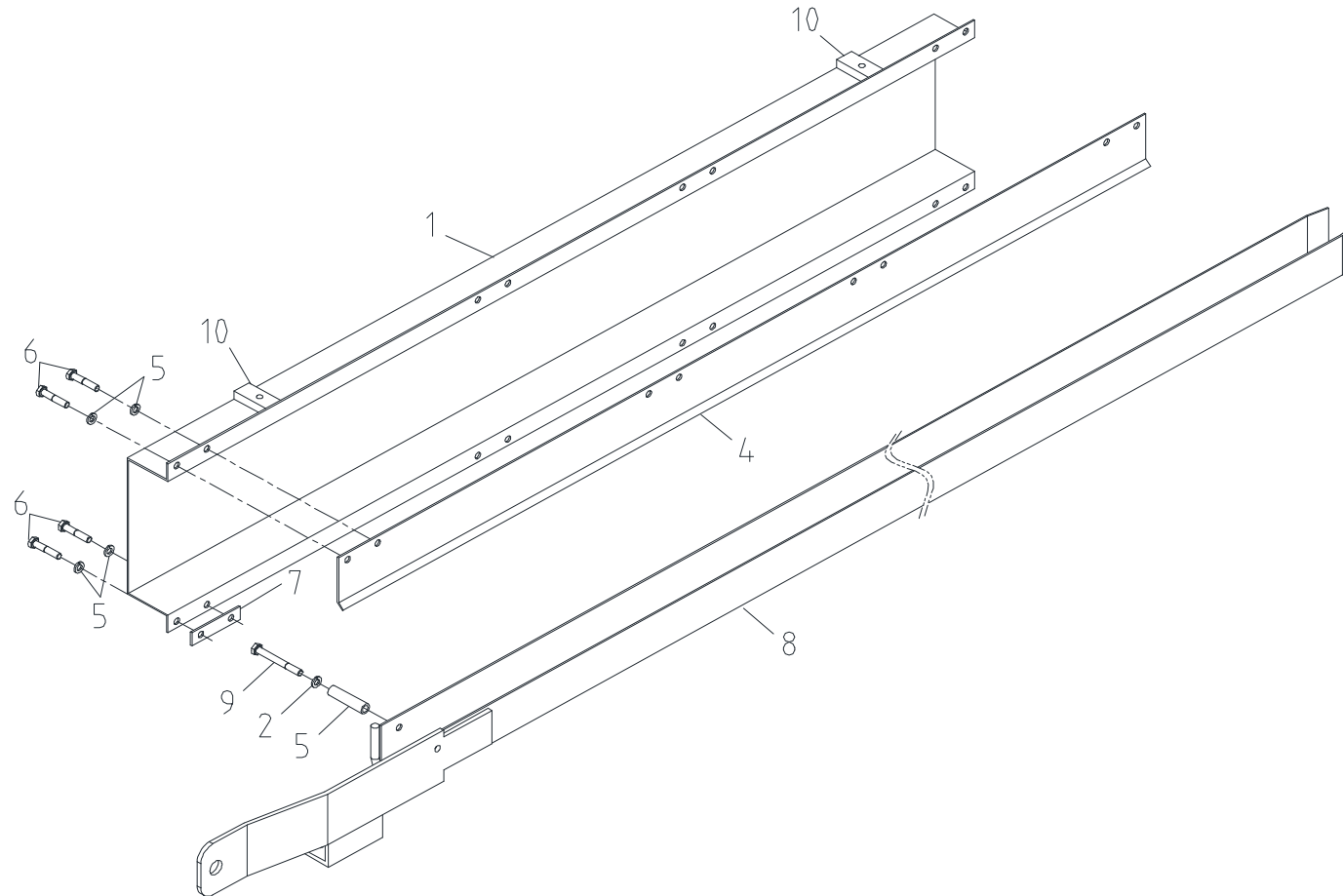
Fig. 1-3 SAC-2501R HOSE GUIDE ASS'Y
