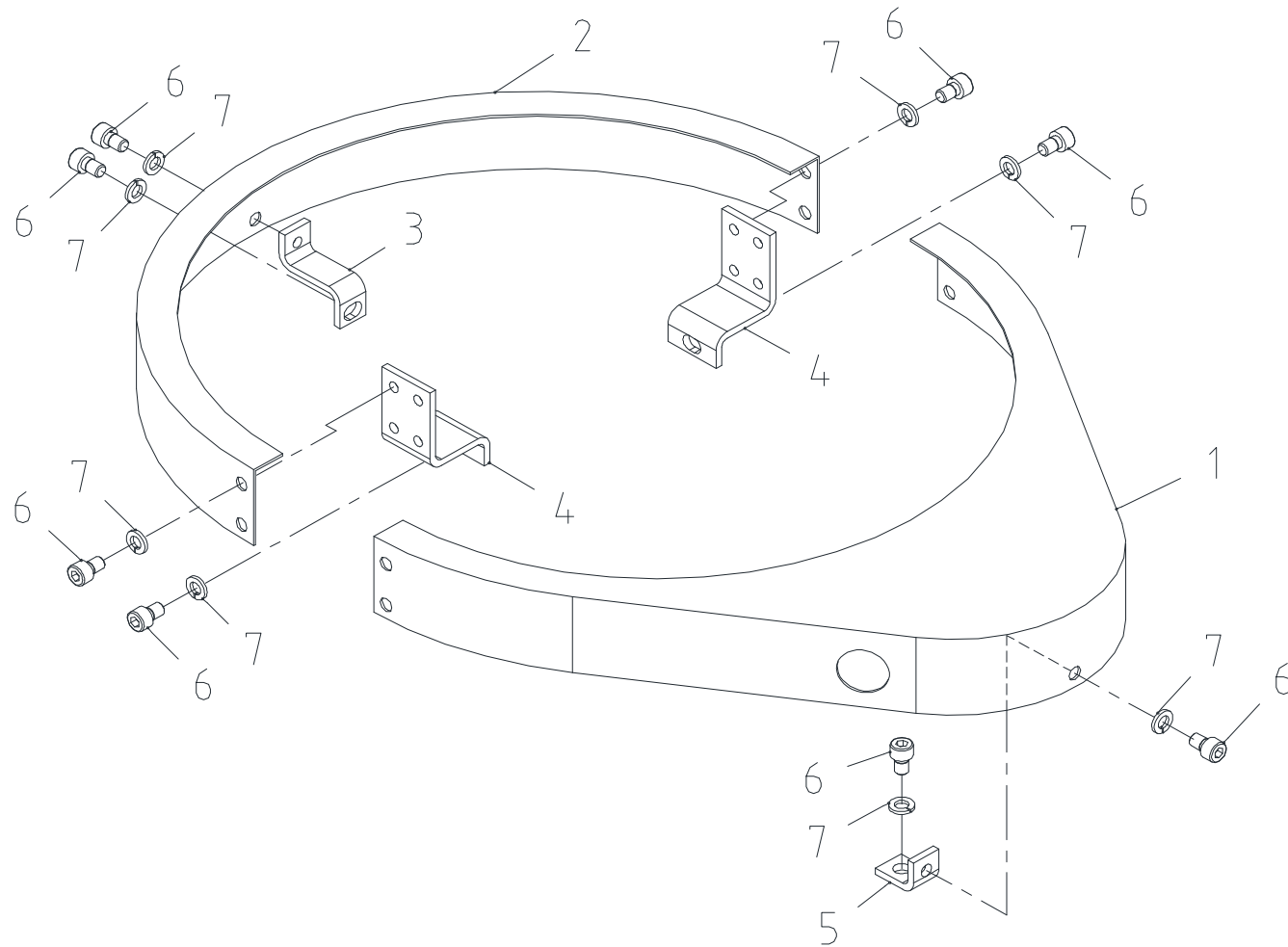
Fig. 2-1-3 SAC-2501R GEAR COVER ASS'Y
