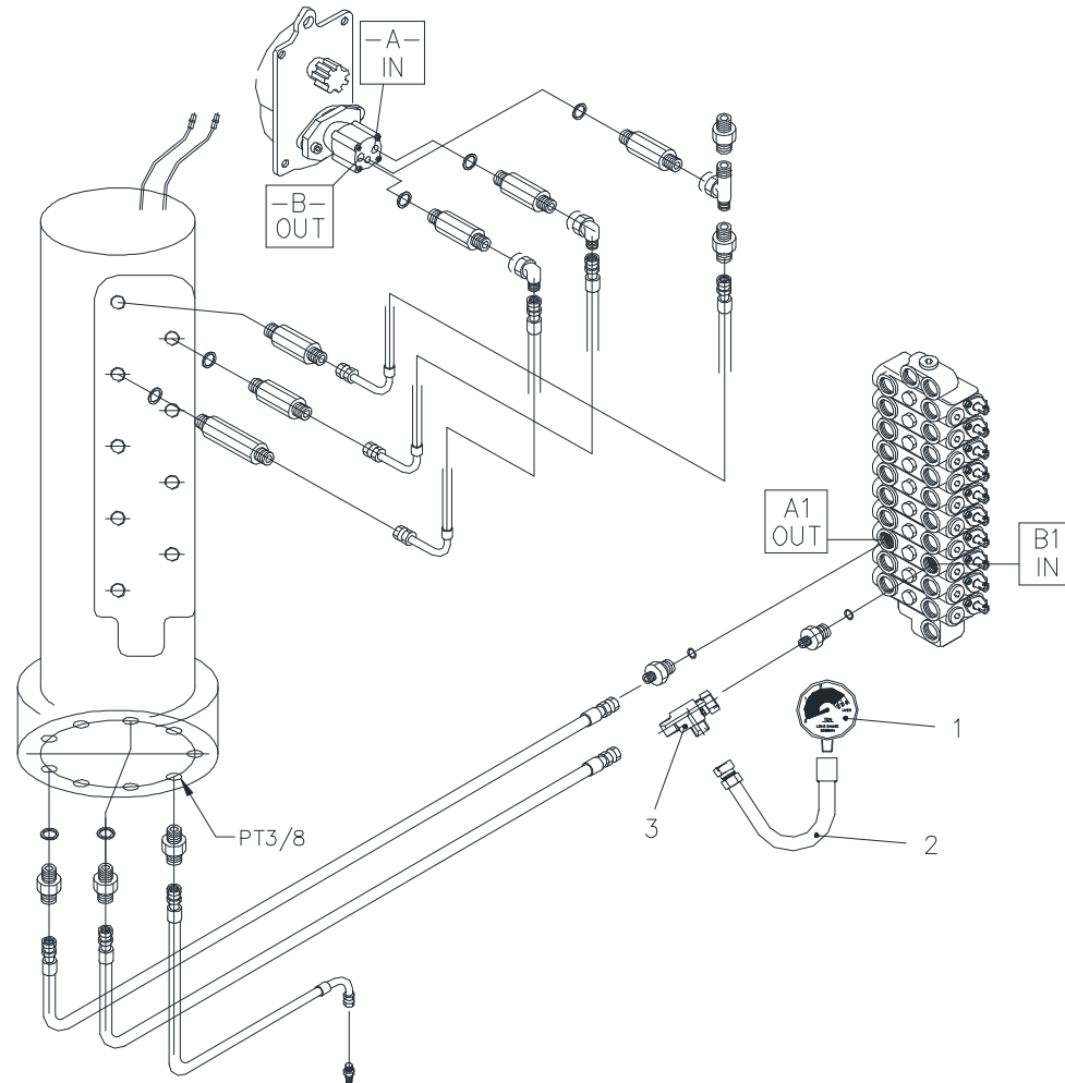
Fig. 4-11 SAC-2501R LOAD GAUGE PIPING
