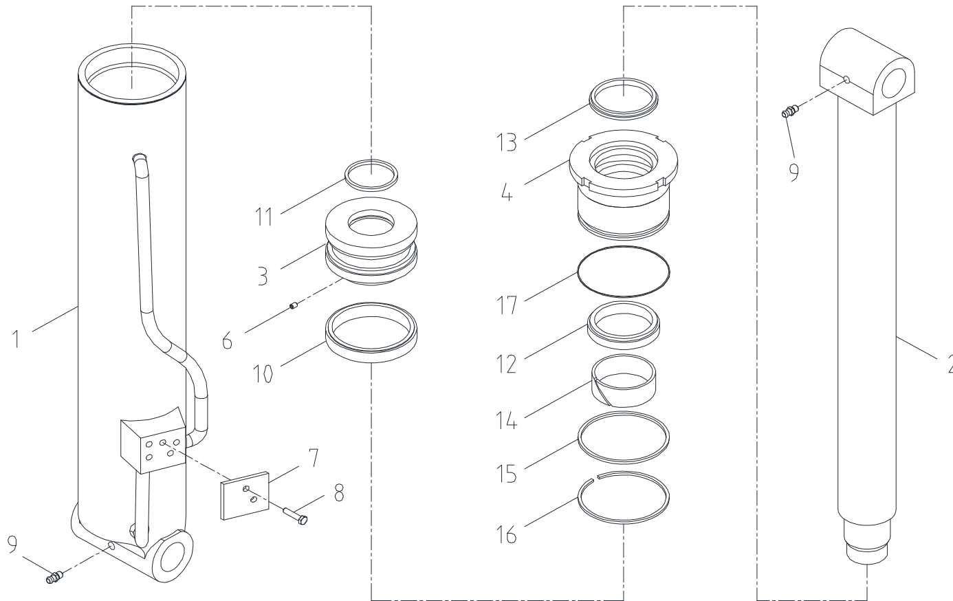
Fig. 2-2-1 SAC-2501R DERRICK CYL'D ASS'Y
