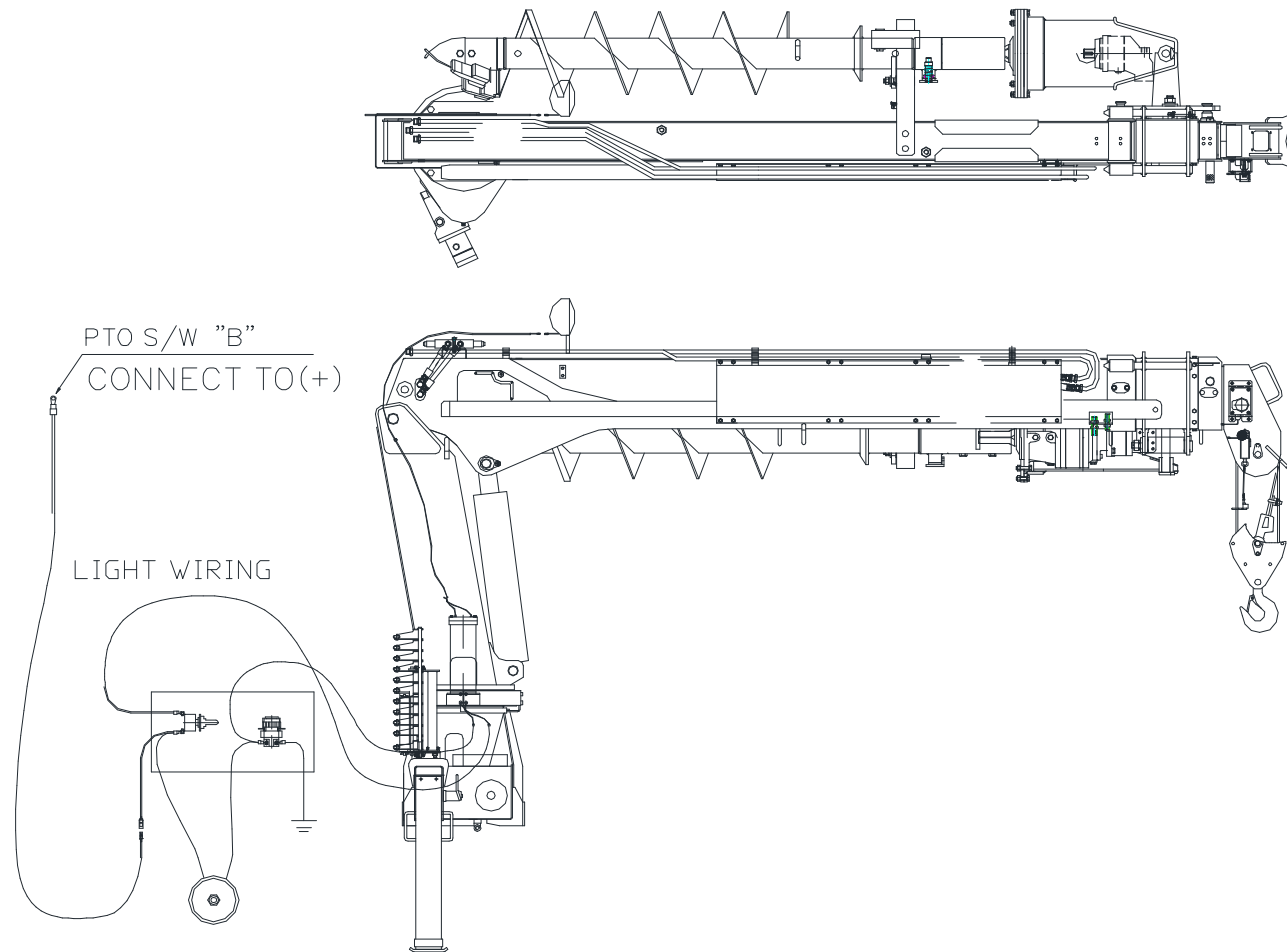
Fig. 11 SAC-2501R ELECTRIC DEVICE
