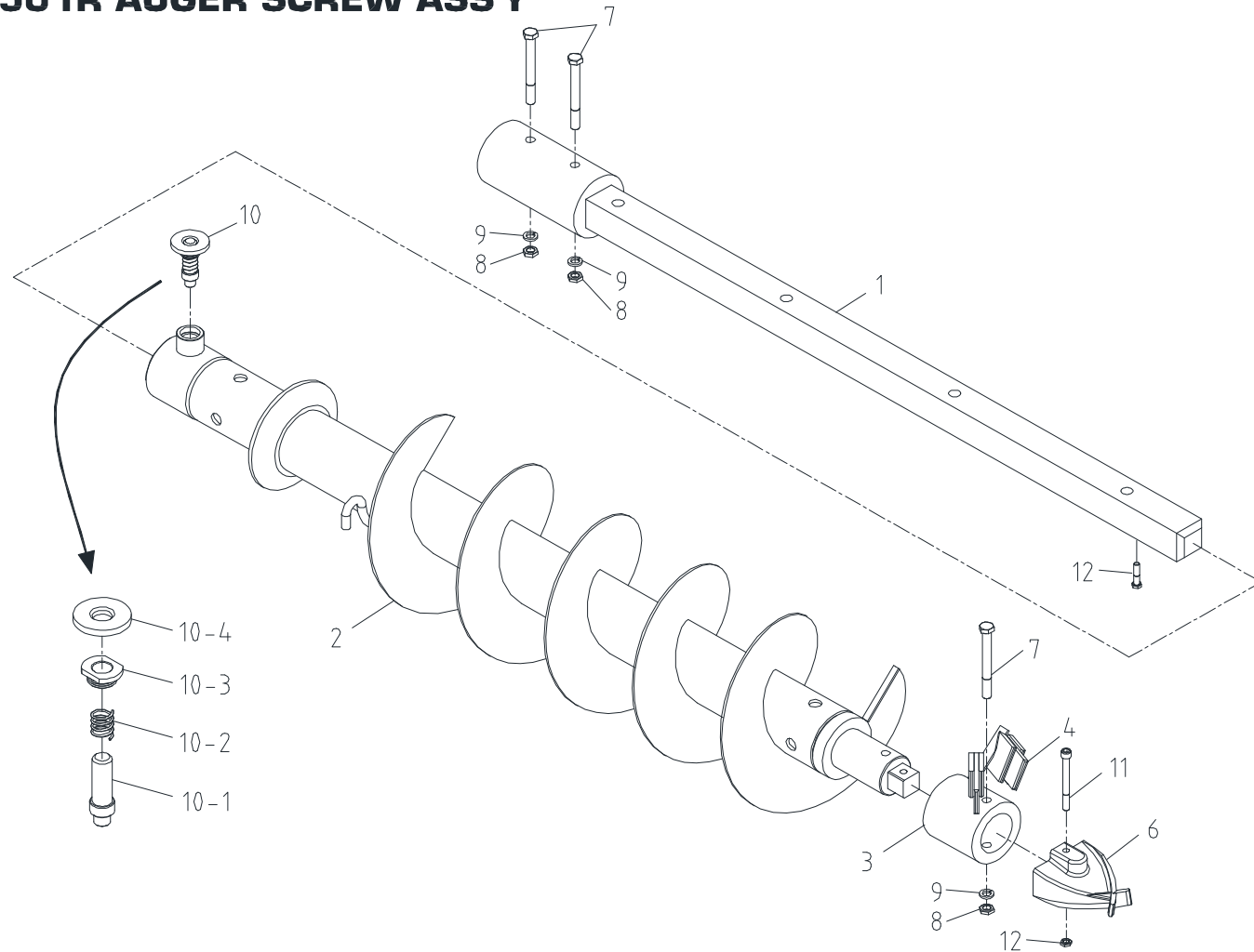
Fig. 5-2 SAC-2501R AUGER SCREW ASS'Y
