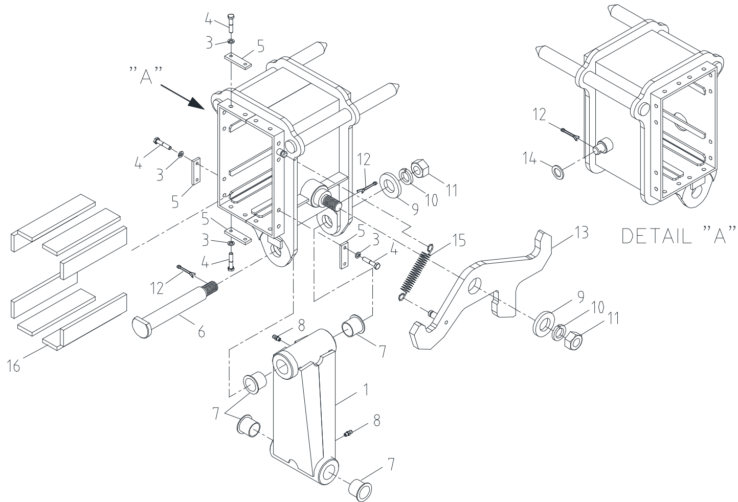
Fig. 1-1 SAC-2501R WORKING BOOM ASS'Y
