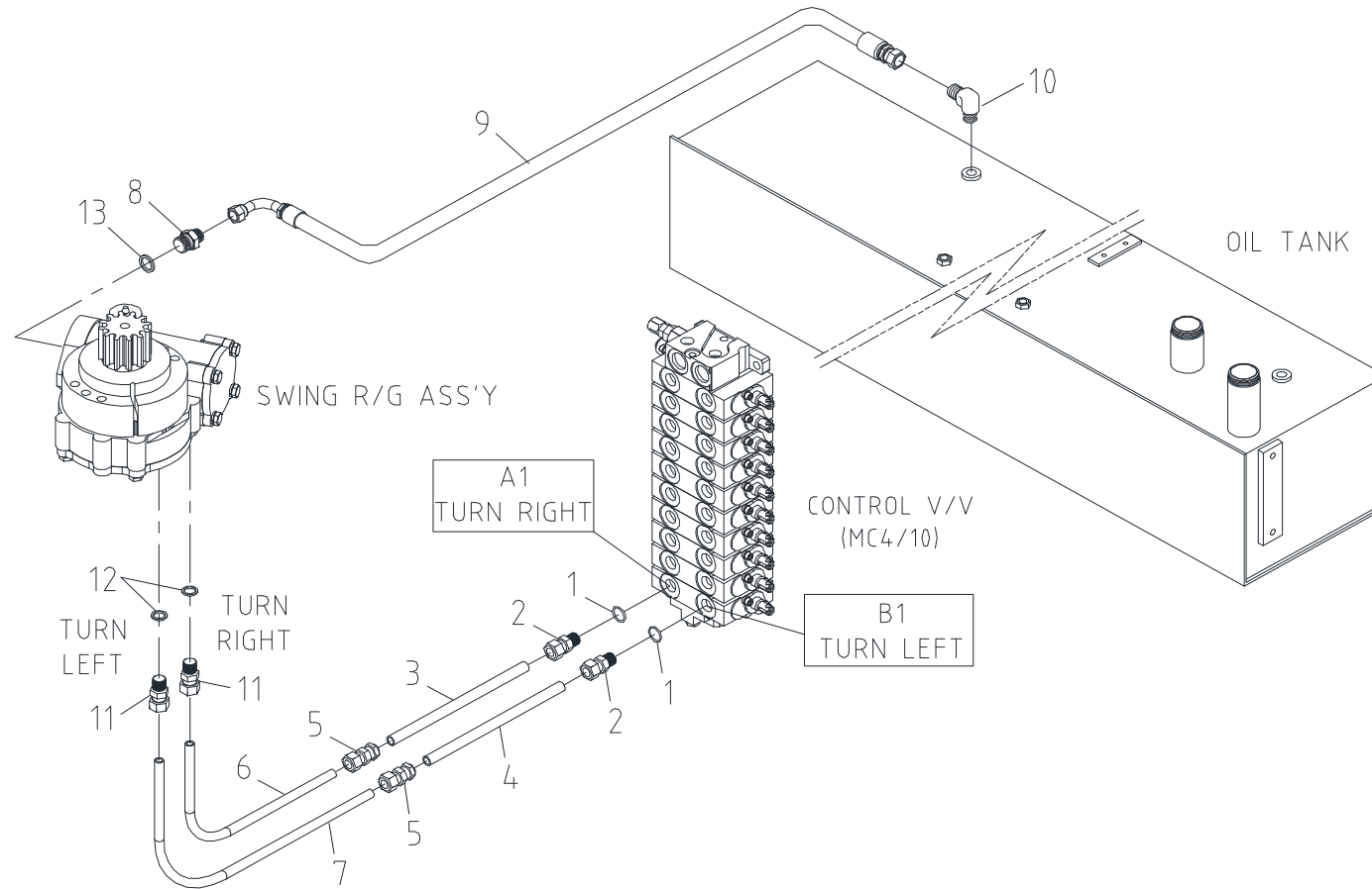
Fig. 4-5 SAC-2501R SWING PIPING
