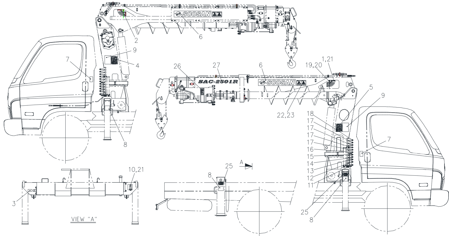
Fig. 6 SAC-2501R STICKER ASS'Y
