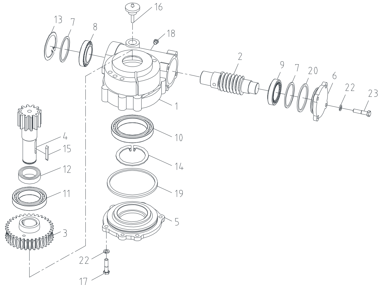
Fig. 2-1-2 SAC-2501R SWING R/G ASS'Y
