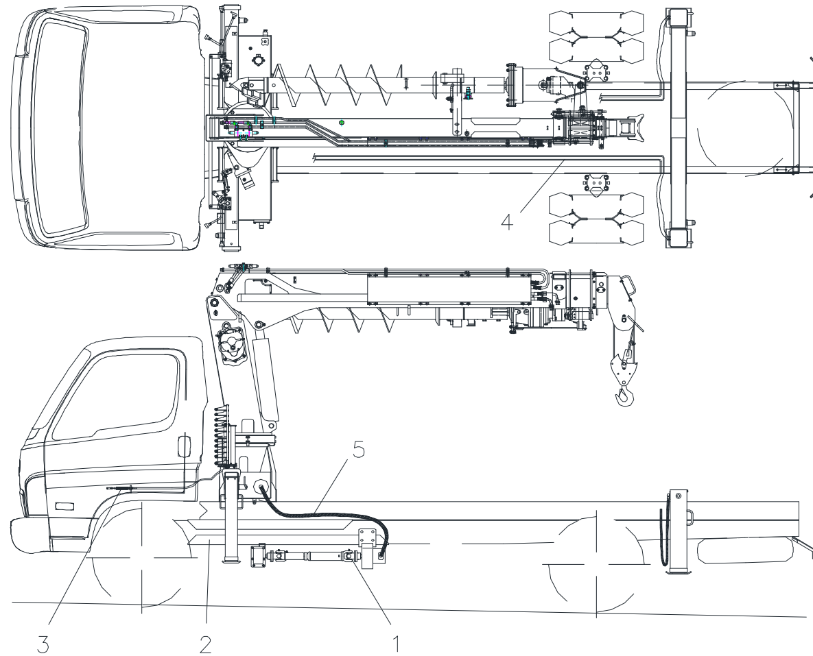
Fig. 8 SAC-2501R MOUNTING ASS'Y
