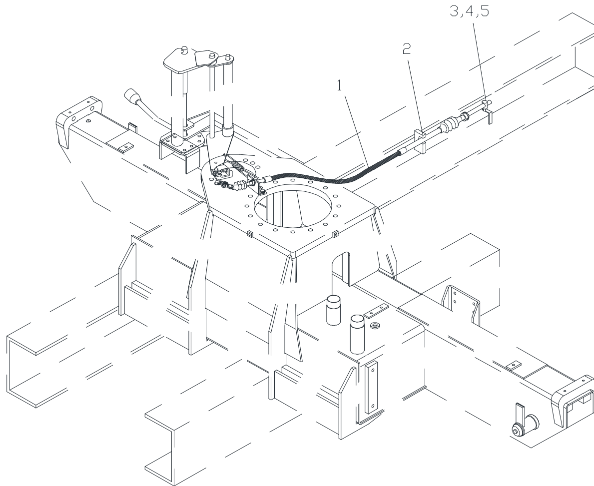
Fig. 8-3 SAC-2501R ACC'L SYSTEM PART
