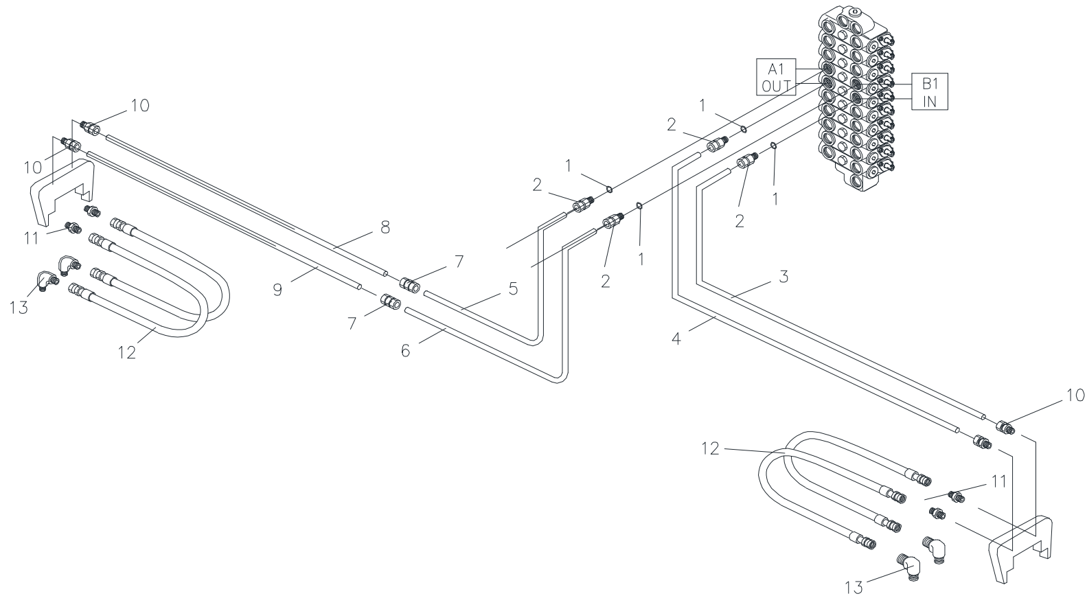
Fig. 4-6 SAC-2501R OUTRIGGER PIPING
