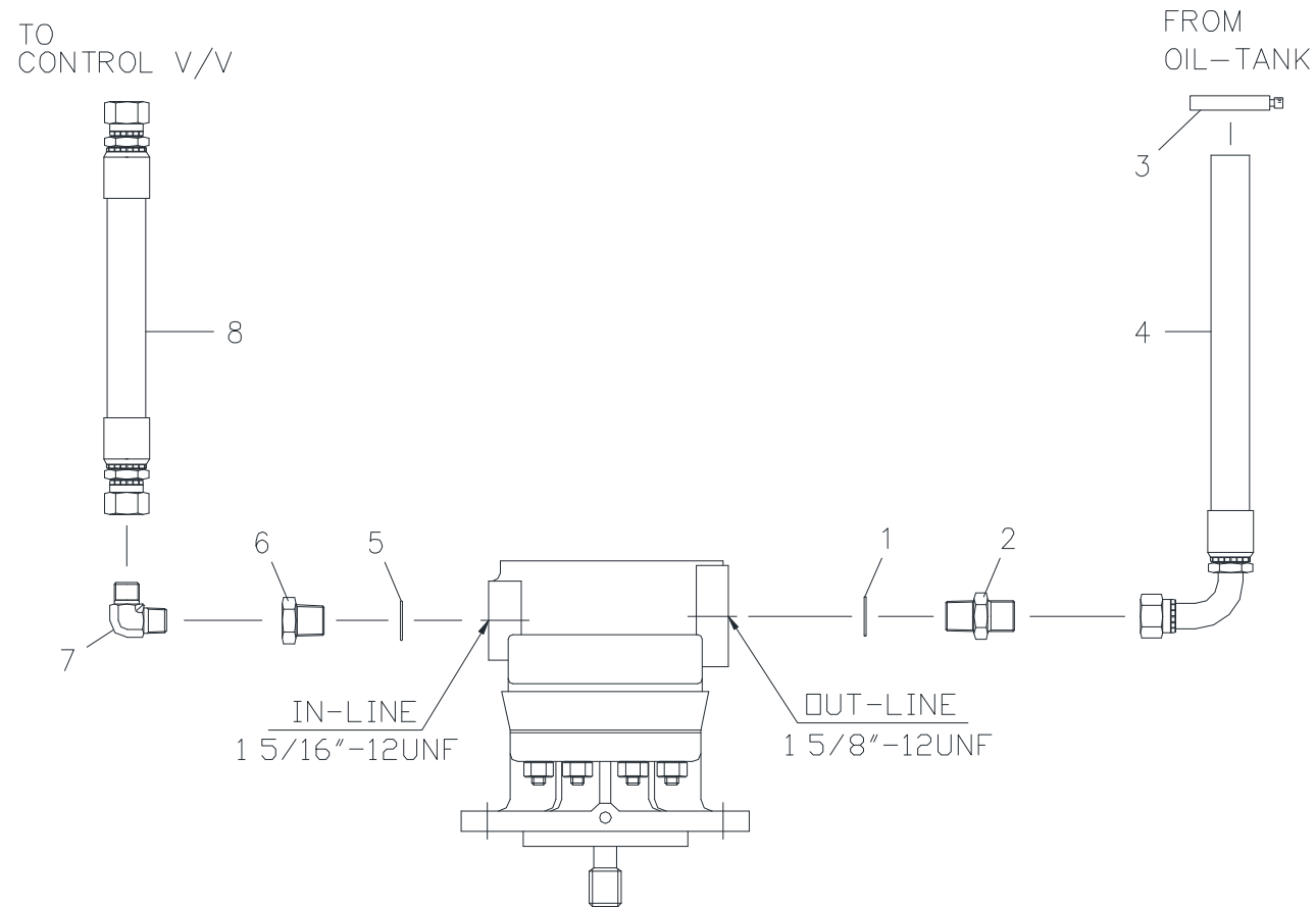
Fig. 8-5 SAC-2501R M/T PIPING PART
